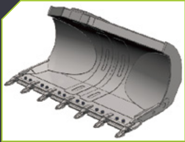
Side dump bucket
